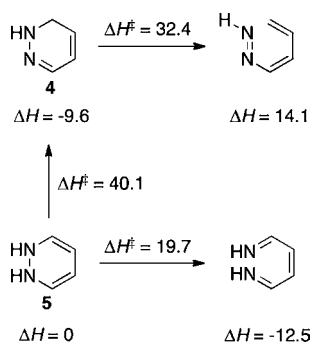
Figure 1. CCSD(T)/cc-pVTZ//B3LYP/6-31G(d) relative enthalpies and enthalpies of activation, both in kcal/mol.
