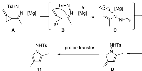
Scheme 3. Proposed Reaction Mechanism
