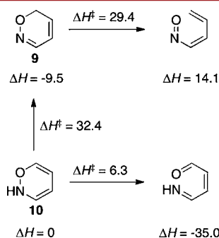
Figure 2. CCSD(T)/cc-pVTZ//B3LYP/6-31G(d) relative enthalpies and enthalpies of activation, both in kcal/mol.
